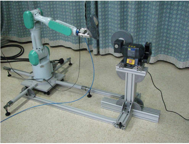
Figure 3: Experimental cell for shoe bottom roughing
